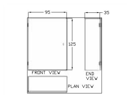
# 382076 - East Coast Type Standard Red Emperor Fire Hose Reel Box Exposed (Painted).
