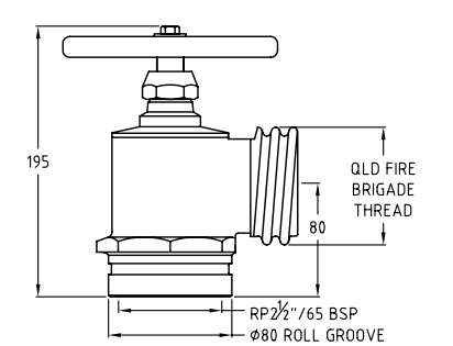
# 381297RGRE - Red Emperor BS Fire Hydrant Valve QLD Thread Round (QLD) Painted - Roll Groove Inlet with Plastic Cap.
