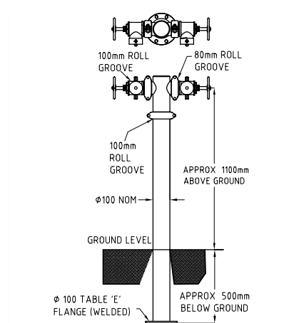
# 381332 - Hydrant Pipe Riser Kit With Split T-Head, Roll Groove Qld Valves & Plastic Caps 100TE X 1600 (Galvanised & Painted)
