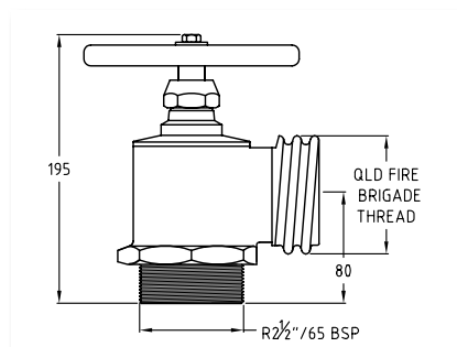
# 381297RE - Red Emperor BS Fire Hydrant Valve QLD Thread Round (QLD) Painted - BSP Inlet with Plastic Cap.
