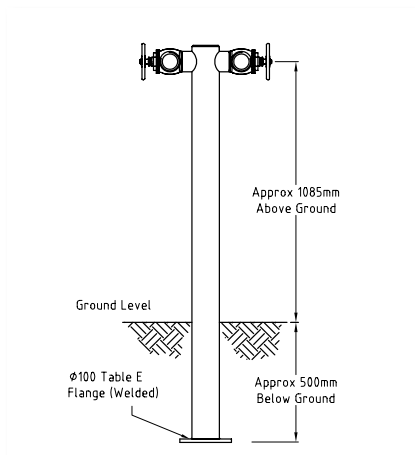
# 381333 - Galvanised Fire Hydrant Pipe Riser Kit with T-Head and QLD Valves (with Plastic Caps), Flanged, Vertical Inlet 100 x 1600 Long (Painted).
