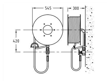
# 383026RE - Red Emperor Fire Hose Reel with Swing Guide Arm 36 mtr.
