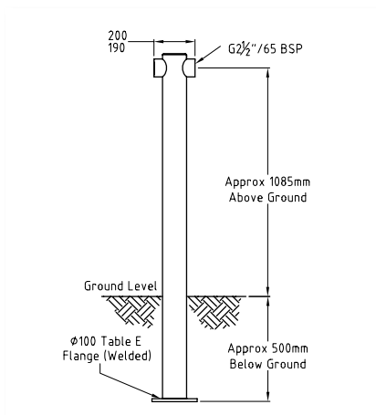
# 381335 - Galvanised Fire Hydrant Pipe Riser with BSP T-Head, Flanged Vertical Inlet 100 x 1600 Long (Painted).
