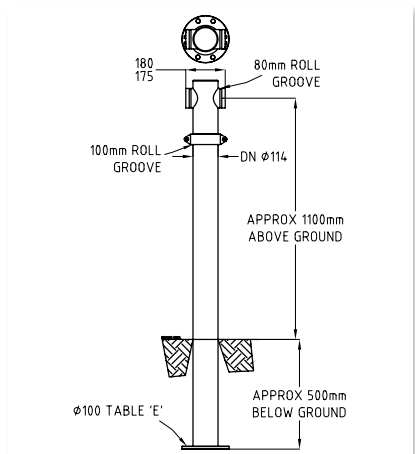
# 381342 - Hydrant Pipe Riser with Split Roll Groove T-Head, Flanged Vertical Inlet 100 X 1600 (Galvanised & Painted)
