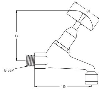
Vandal Resistant Chrome Plated Brass J/V Deluxe Bib Tap Aerated - Hot
