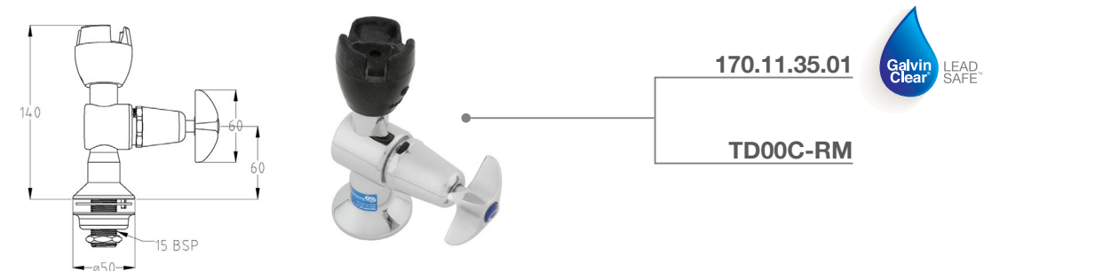
Ezy-Drink® Chrome Plated Brass Vertical Cam Action Drinking Bubbler Tap RH - MI
