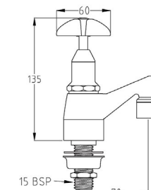
Vandal Resistant Chrome Plated Brass J/V Pillar Tap (NSW) Cold with Vandal Resistant 8 LPM Aerator
