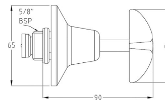
Vandal Resistant Chrome Plated Brass J/V Washing Machine Tap - Cold
