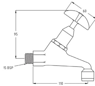
Vandal Resistant Chrome Plated Brass J/V Deluxe Bib Tap (NSW) Cold with 8LPM Aerator
