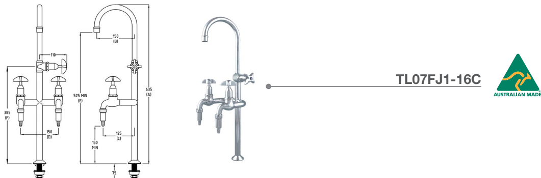
GalvinLab® Chrome Plated Brass Lab Set 3-Way Type 7 Fixed J/V #1 Aerator & #16XT Tube Nozzle
