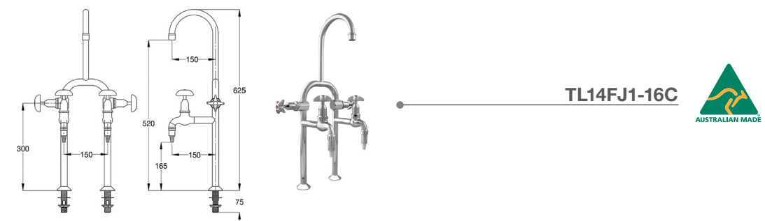
GalvinLab® Chrome Plated Brass Lab Set H&C Mixing Unit Type 14 Fixed J/V #1 Aerator & #16XT Tube Nozzle
