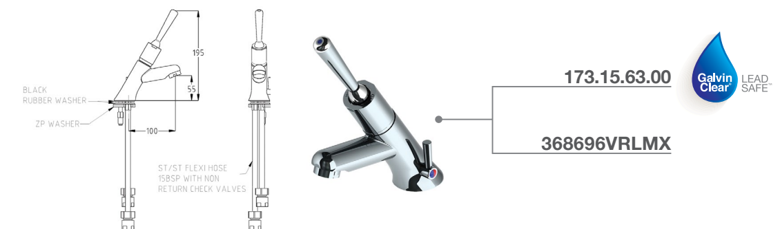
Ezy-Lever Chrome Plated Brass Timeflow Lever Action Vandal Resistant Pillar Tap - Temperature Mixing
