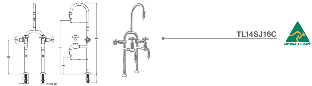
GalvinLab® Chrome Plated Brass Lab Set H&C Mixing Unit Type 14 Swivel J/V #16XT Tube Nozzle
