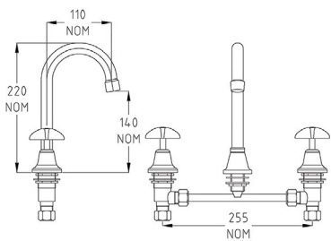
Vandal Resistant Chrome Plated Brass J/V Basin Set (NSW) with Vandal Resistant 6LPM Aerator
