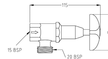
Vandal Resistant Chrome Plated Brass J/V Washing Machine Tap - Hot
