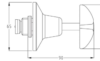
Vandal Resistant Chrome Plated Brass Wall Top Assembly with Jumper Valve - Hot
