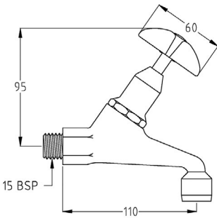
Vandal Resistant Chrome Plated Brass J/V Basin Set (NSW) with Vandal Resistant 6LPM Aerator
