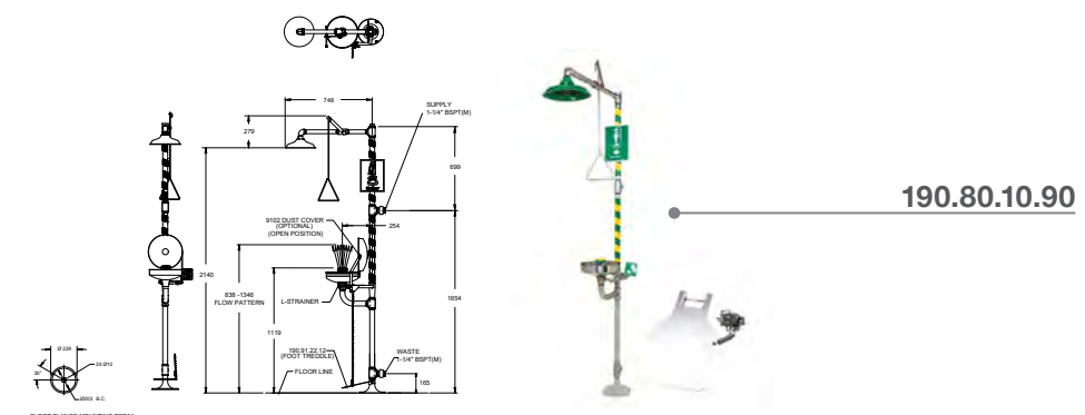
GalvinSafe® Free Standing Combi Shower, Eye/Face Wash, Hand & Foot Act, Axion® ABS Shower
