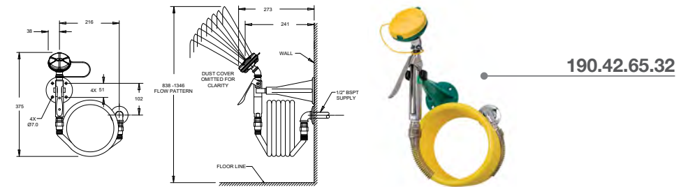
GalvinSafe® Body Spray, Wall Mounted, Hand Held, 2.4mtr Pressure Hose (HAWS)
