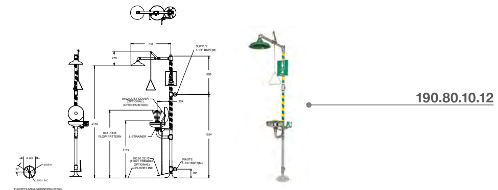
GalvinSafe® Free Standing Combi Shower, Eye/Face Wash, Hand Act, Axion® ABS Shower (HAWS)
