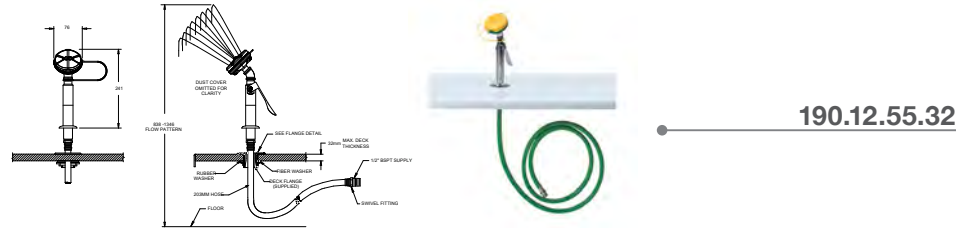
GalvinSafe® Drench Shower, Wall Mounted, Pull Rod, Axion® ABS Shower (HAWS)
