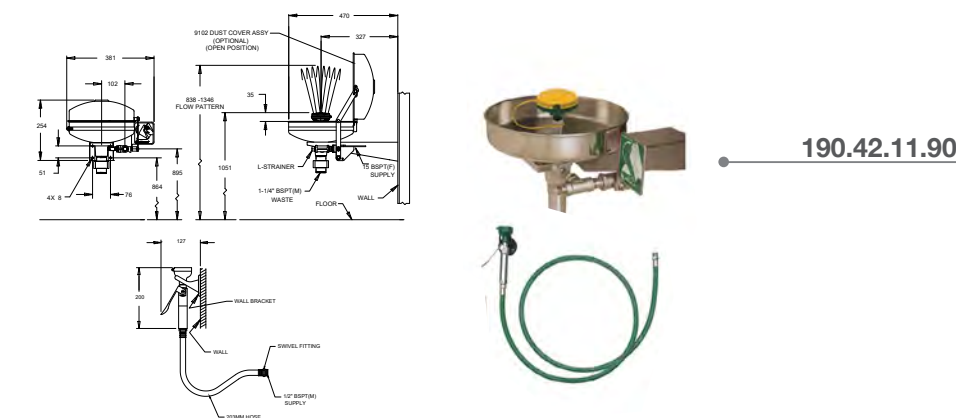
GalvinSafe® Eye/Face Wash, Wall Mtd, Hand Act, Axion® ABS Bowl, Hand Held Drench Hose (HAWS)
