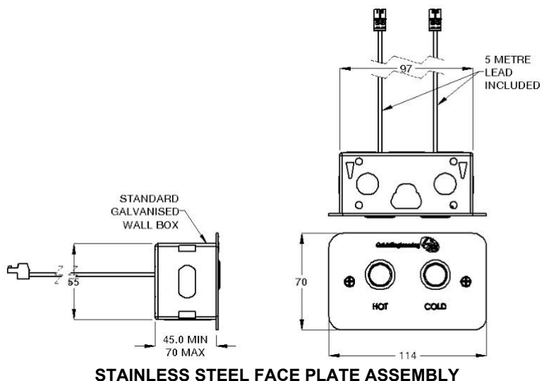
STAINLESS STEEL FACE PLATE ASSEMBLY
