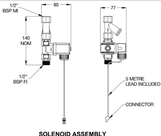
SOLENOID ASSEMBLY
