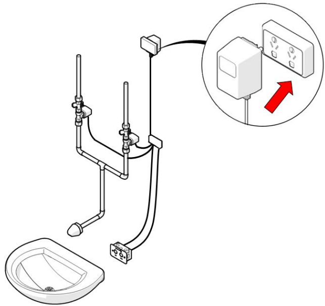
Typical Installation
