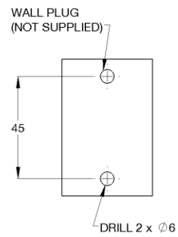
Rough-In Dimensions
