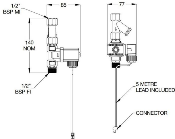
SOLENOID ASSEMBLY
