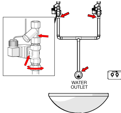
Typical Installation
